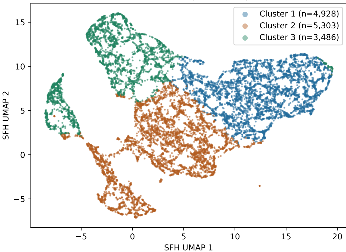
KMeans in full aligned SFH space
