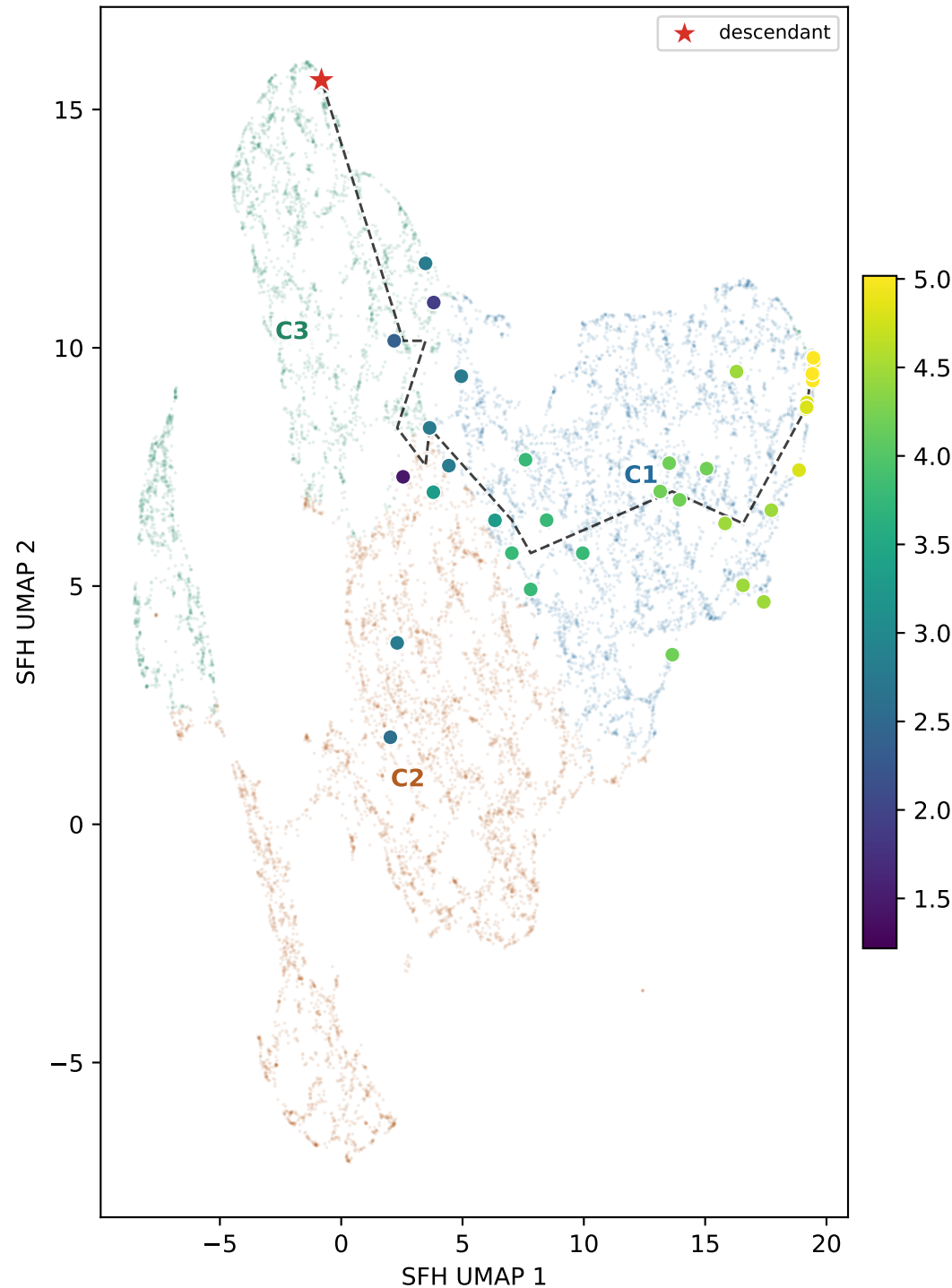
Analogue positions and fixed SFH-cluster regions
