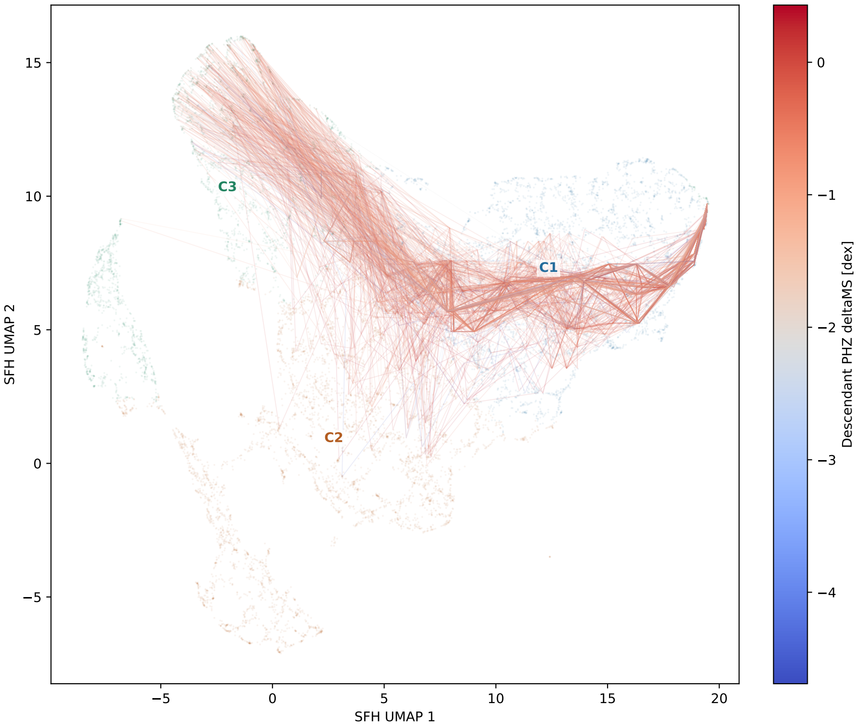
All analogue-centroid tracks Color encodes descendant PHZ deltaMS
