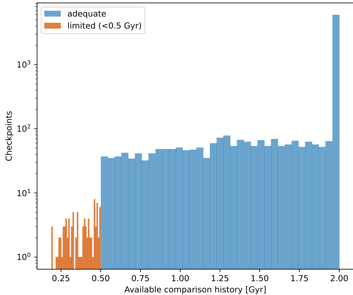
History available for SFH matching
