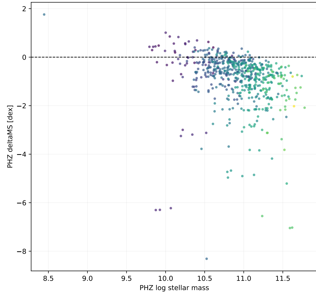
No descendant mass cut
