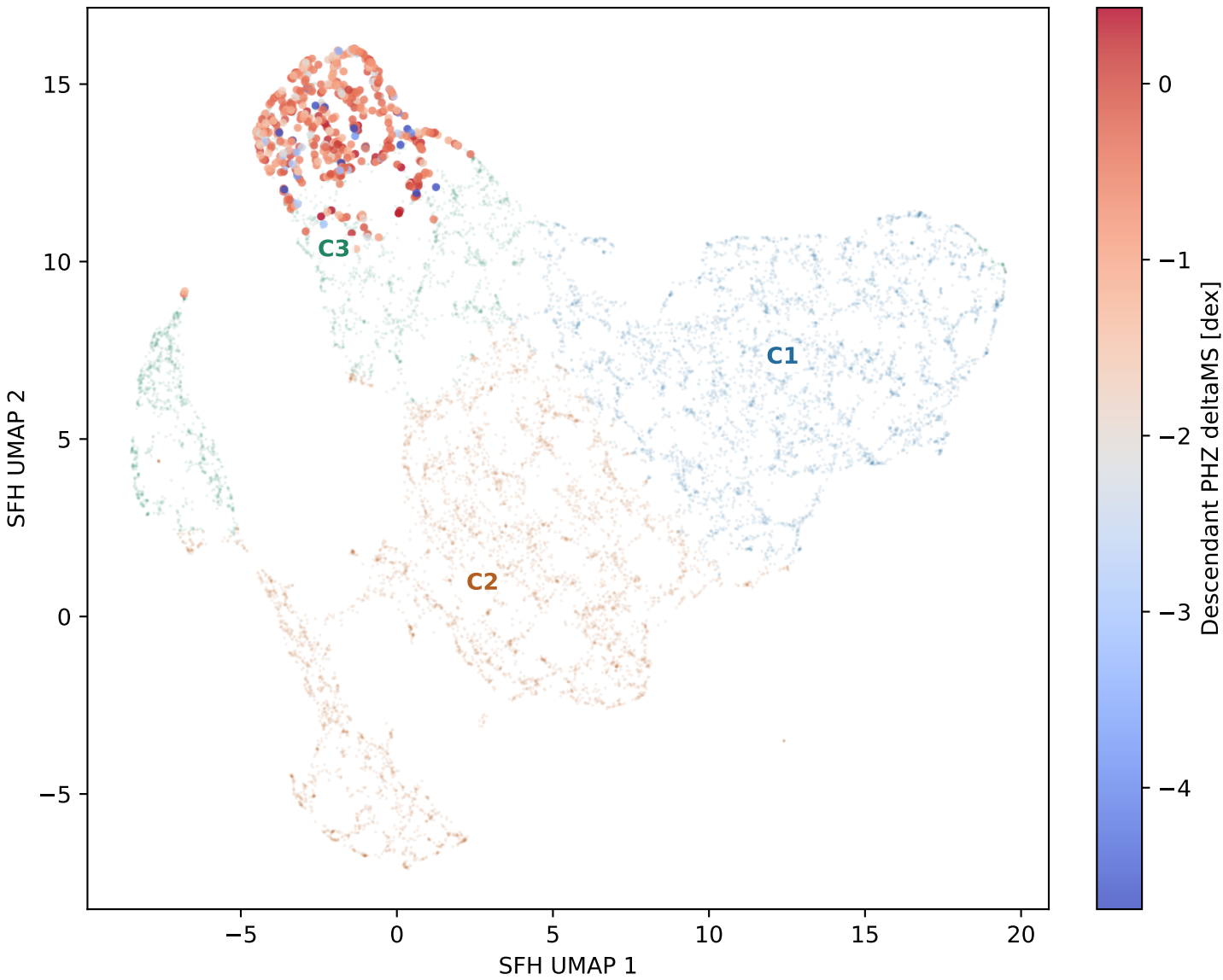
All 587 selected descendants
