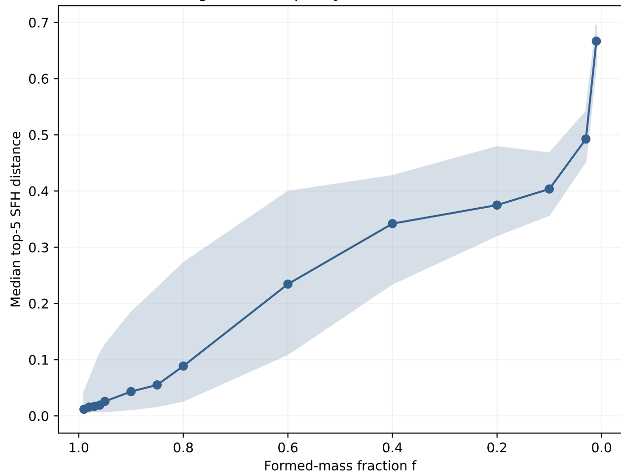
Analogue-match quality across all descendants
