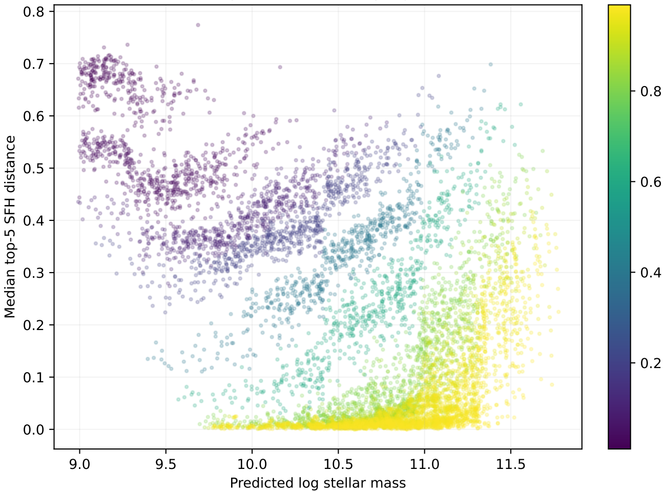
Match quality versus inferred progenitor mass
