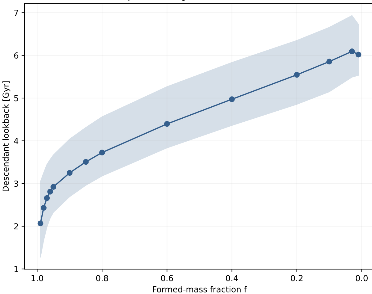
Checkpoint timing across all descendants
