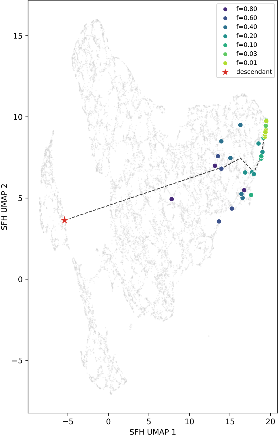
Analogue positions after SFH-only selection
