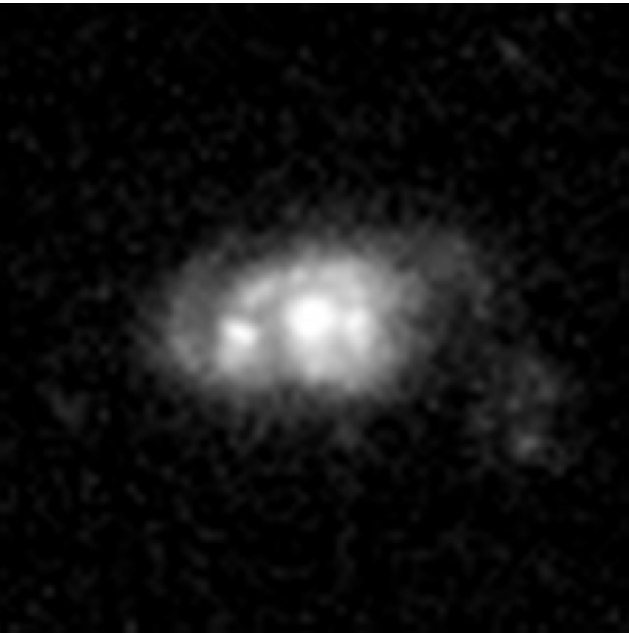
Descendant 2648419808652582361 log M*=11.00, z=0.810
