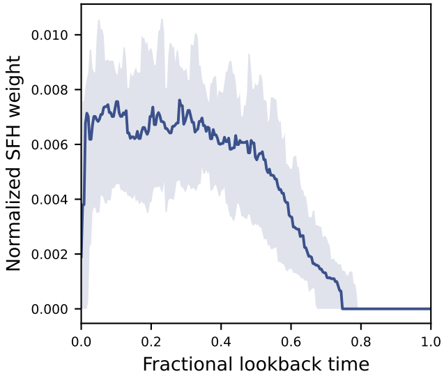
Complete candidate SFH
