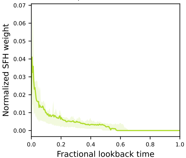
Complete candidate SFH
