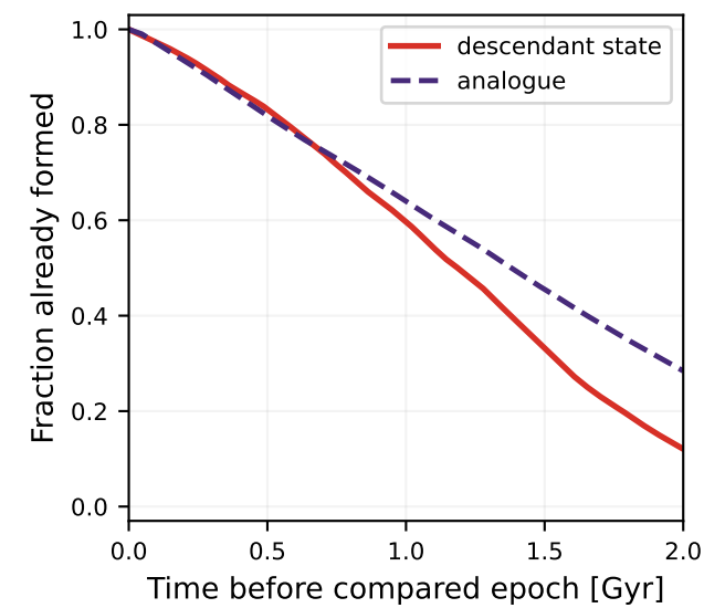
Fractional lookback time
