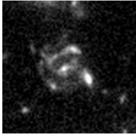
Complete candidate SFH
