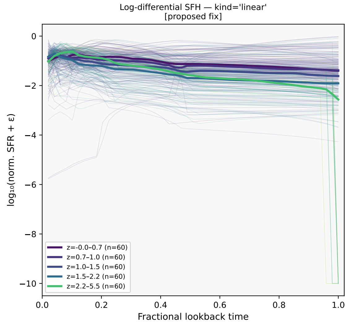
SFH representations coloured by redshift (N=300)
