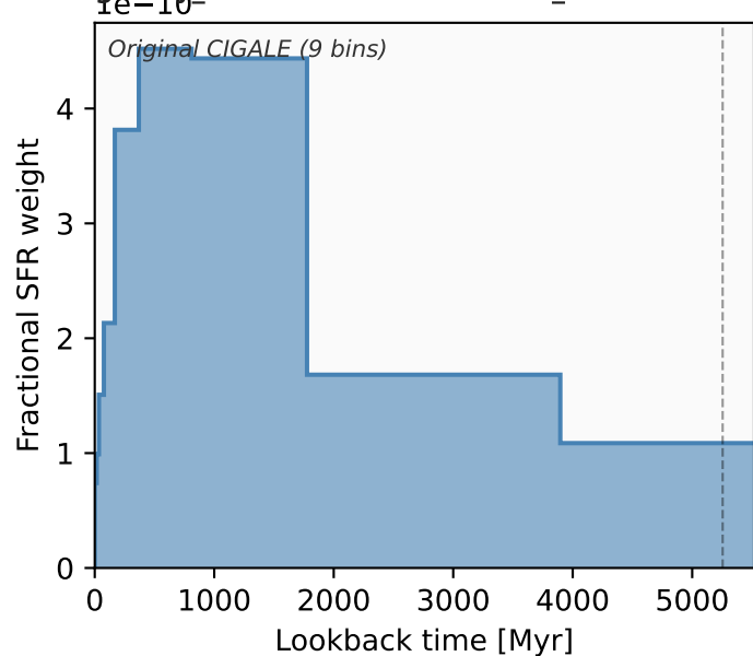
galaxy_id=604721 z=1.134 t_univ=5255 Myr
