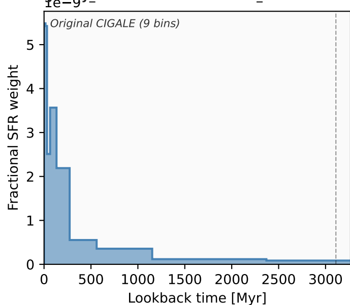
galaxy_id=723676 z=2.076 t_univ=3110 Myr
