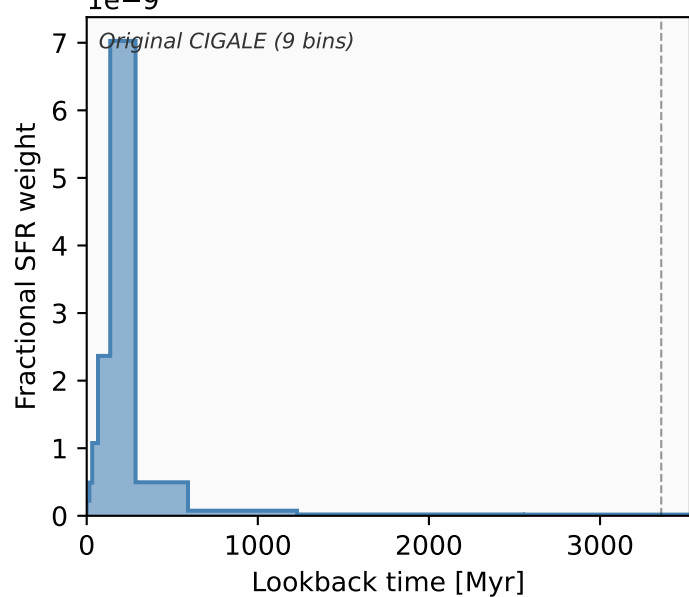
galaxy_id=565802 z=1.919 t_univ=3358 Myr
