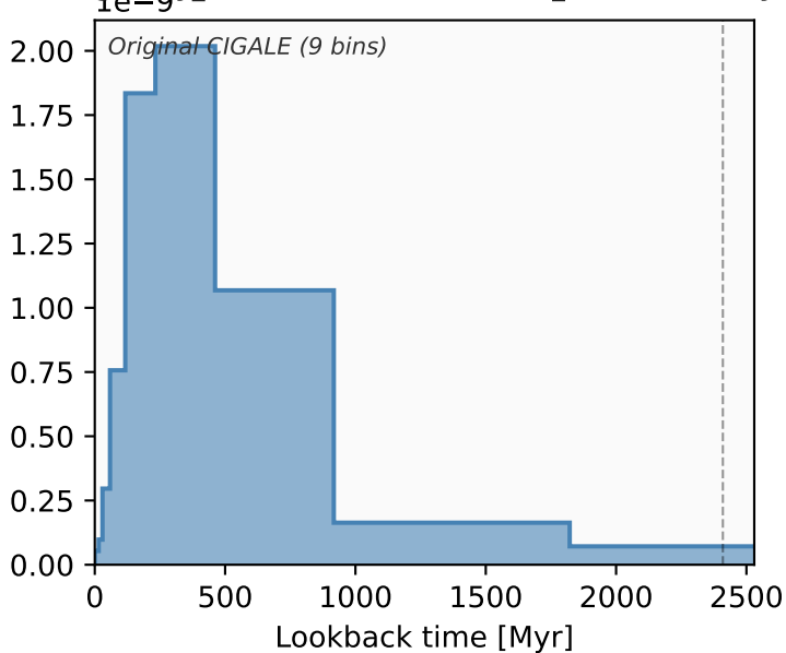
galaxy_id=626452 z=2.660 t_univ=2410 Myr
