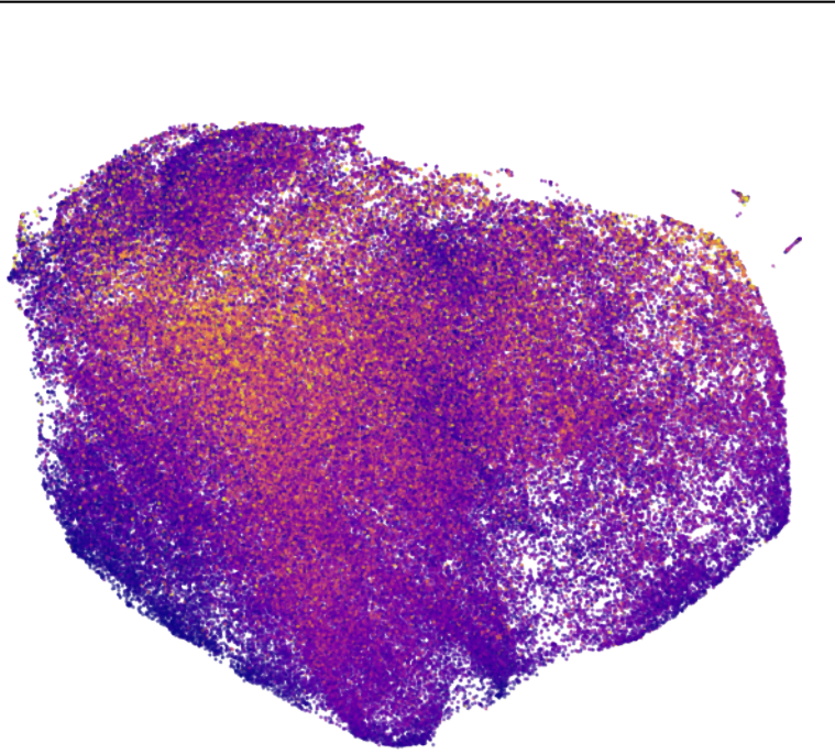
Image (ZooBOT)
