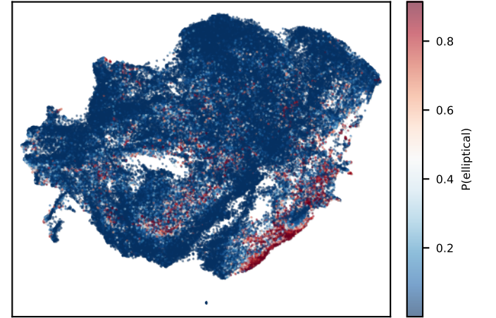
P(elliptical)
