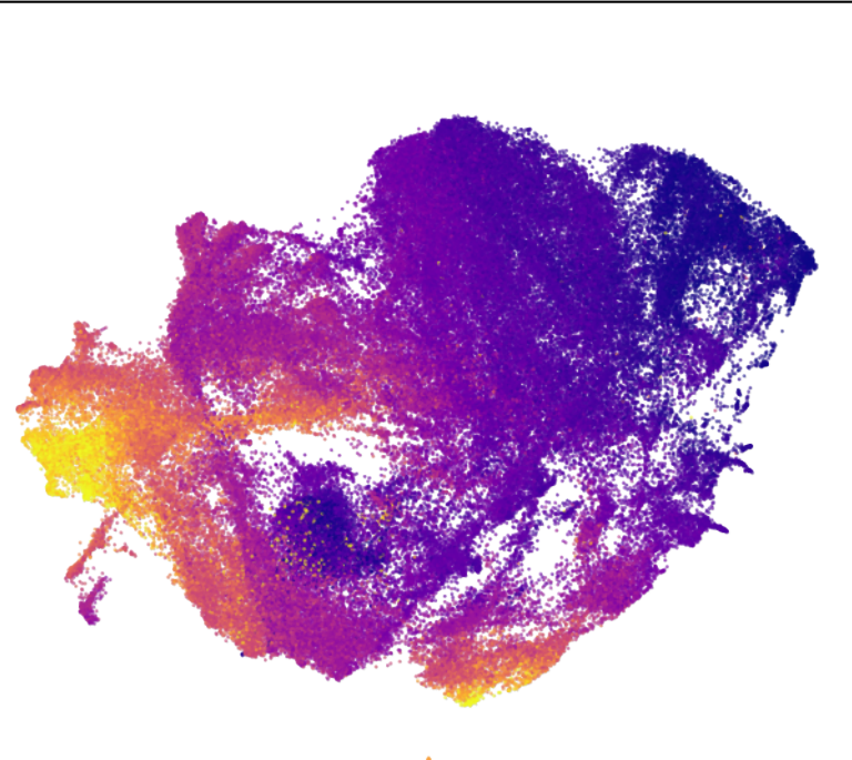
Joint (avg)
