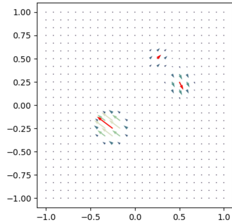
RBFVec(variance=1.0, lengthscale=0.1)
