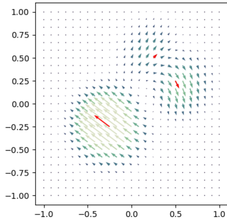
RBFVec(variance=1.0, lengthscale=0.25)
