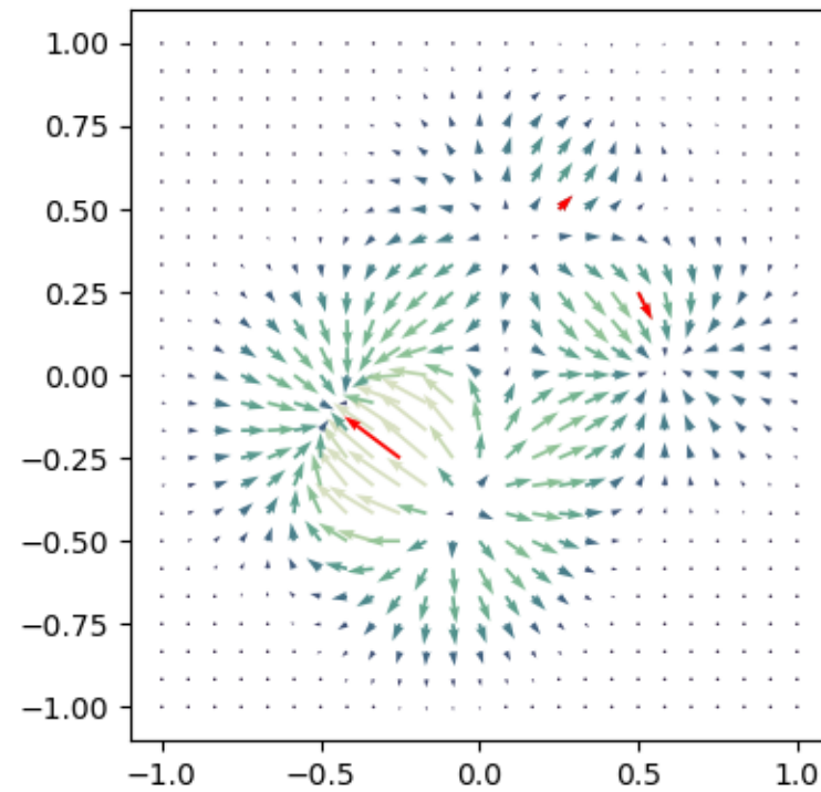
RBFDivFree(variance=1.0, lengthscale=0.25)
