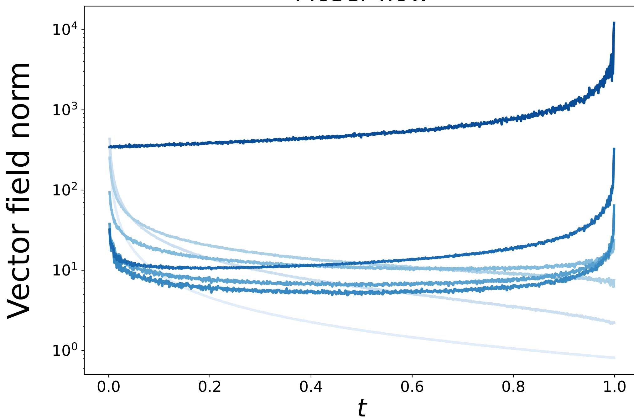
Moser flow
