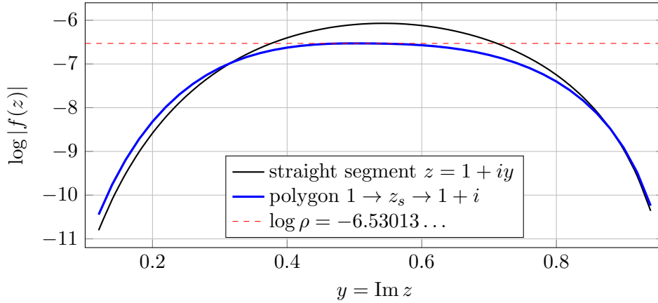
FIGURE 2. The size of f along the upper half of the two paths, as a function of y = \operatorname{Im} z (the lower half is the mirror image; at the zeros z = 1 and z = 1 + i of f the curves go to -\infty ). On the straight segment the maximum of \log |f| is -6.0709 ; on the polygon \log |f| stays below \log \rho (Proposition 7.1), and it comes close to this value only near the vertex z_s , at y = 0.4939 .
