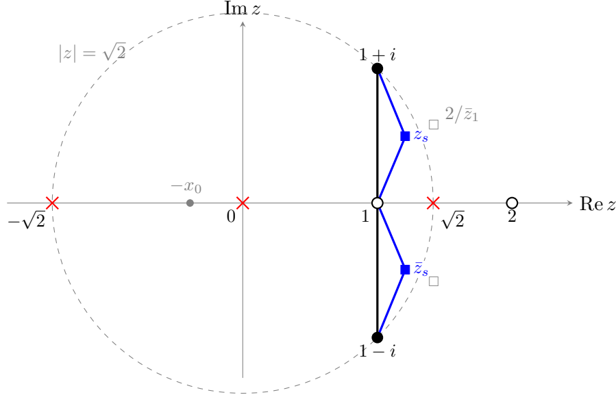
FIGURE 1. The z -plane. Crosses: the poles 0, \pm\sqrt{2} of f . Open circles: the zeros 1, 2 (order 5). Black dots: the zeros 1 \pm i (order 3), which are the end points of the path. Black segment: the path of integration in (1.2). Blue: the polygon 1 - i \rightarrow \bar{z}_s \rightarrow 1 \rightarrow z_s \rightarrow 1 + i of Section 7; its vertex z_s is a rational point at distance less than 10^{-5} from the saddle point z_1 = 1.2077099\dots + 0.4939472\dots i of |f| . The symmetry z \mapsto 2/z maps the dashed circle to itself and z_1, \bar{z}_1 to the saddle points 2/z_1, 2/\bar{z}_1 , which are marked by grey squares. The grey dot is the point -x_0 = -0.39126\dots where |f| is minimal on the interval (-\sqrt{2}, 0) (Section 6).
