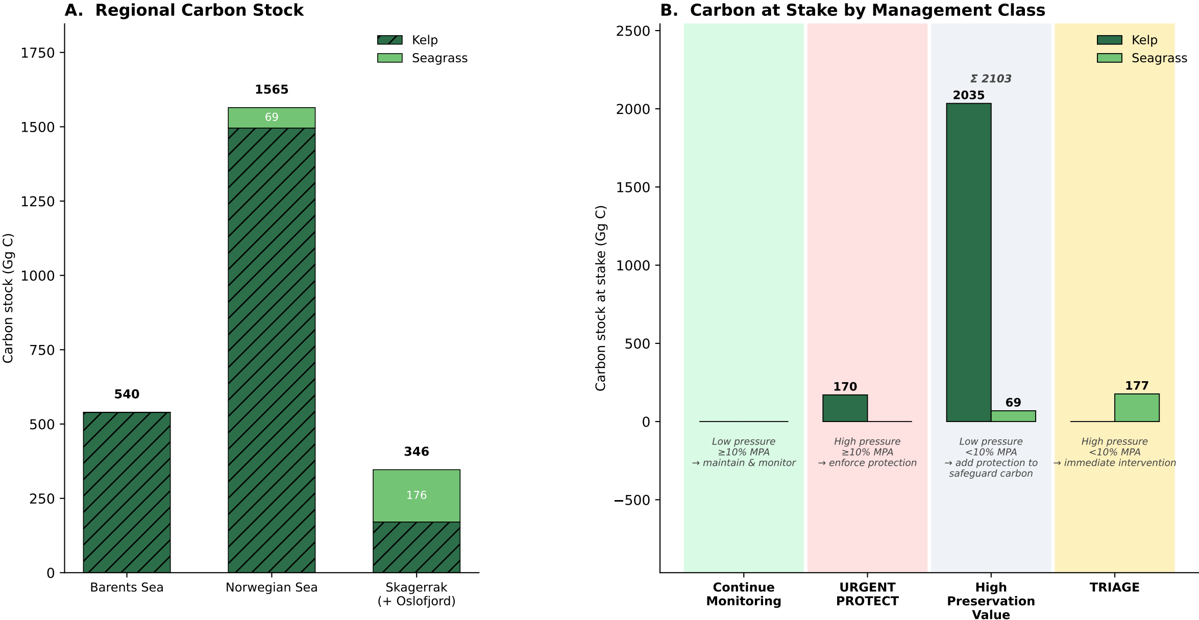
Panel A: Total carbon stock (Gg C) by region; kelp uses national mean density (Gundersen 2021), seagrass uses regional mean density (Gagnon 2024). Hatching = kelp (equal-density assumption). Panel B: Carbon in each management class. Pressure threshold = within-dataset median; MPA adequacy = 10% (policy benchmark). Values in Gg C.
