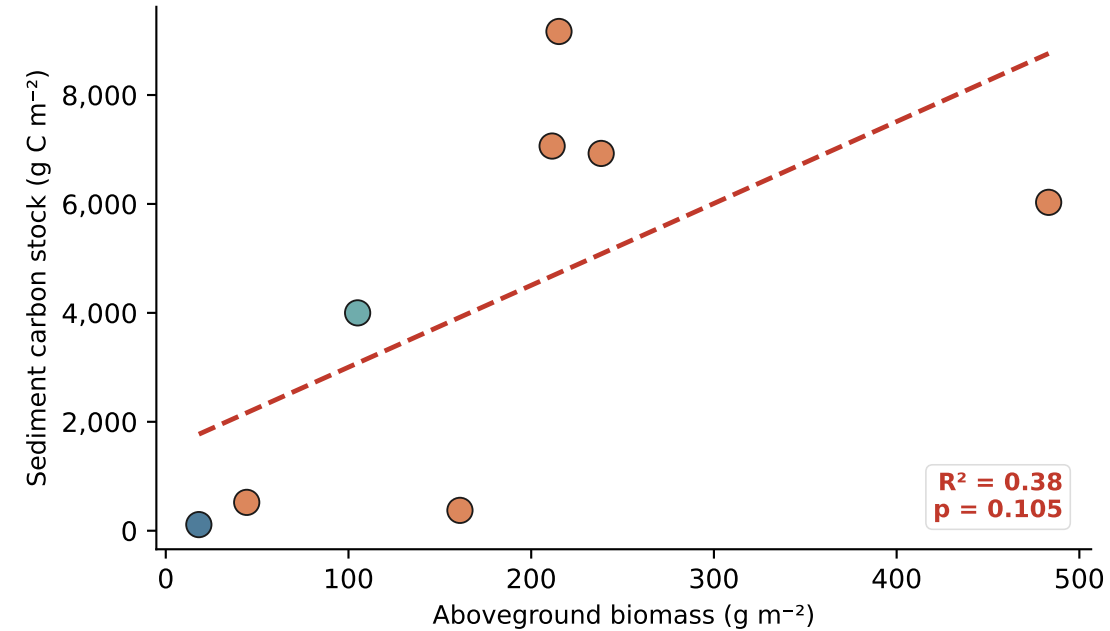
B. Aboveground Biomass
