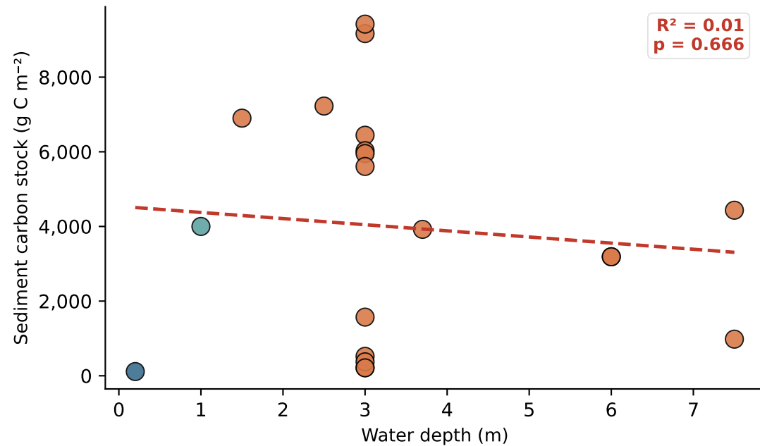
C. Water Depth
