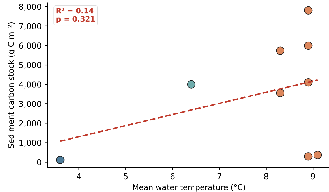
D. Mean Temperature
