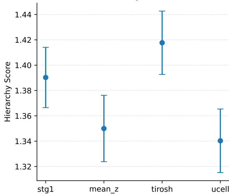
Hierarchy Score
