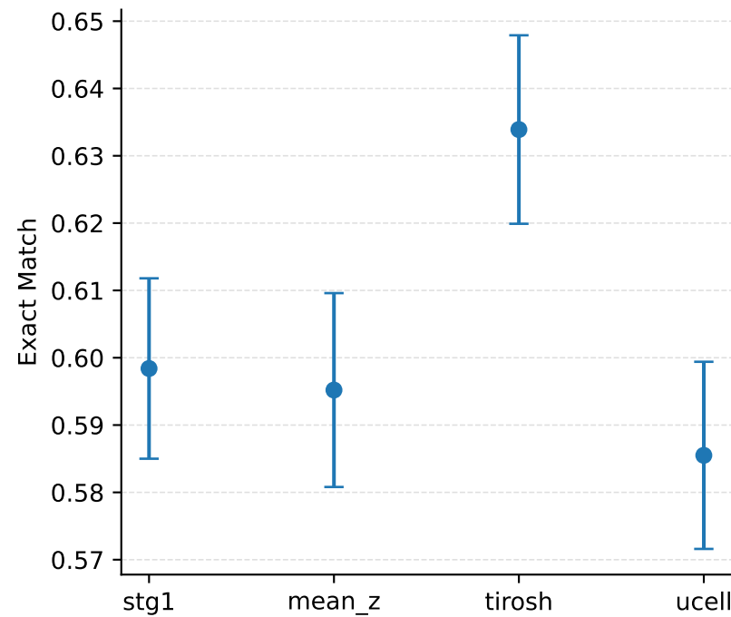
Exact Match
