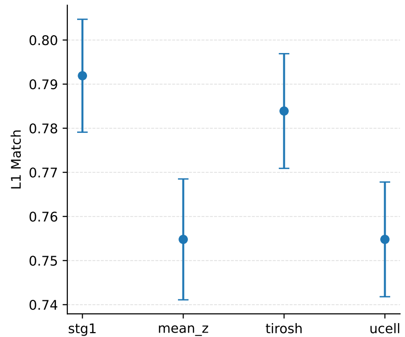
L1 Match
