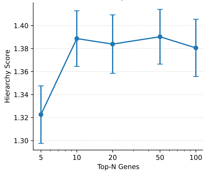
Hierarchy Score
