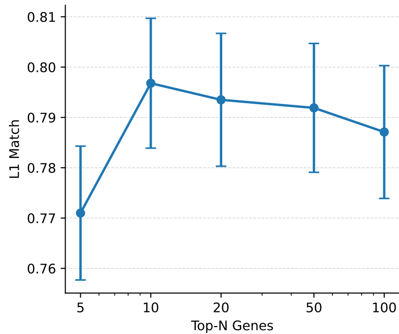
L1 Match
