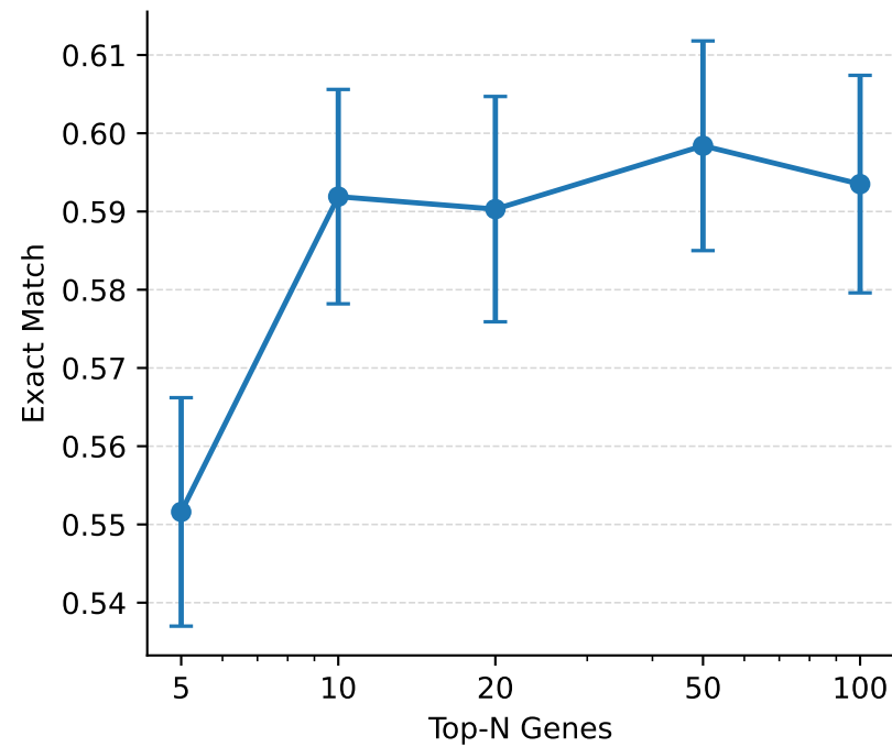
Exact Match
