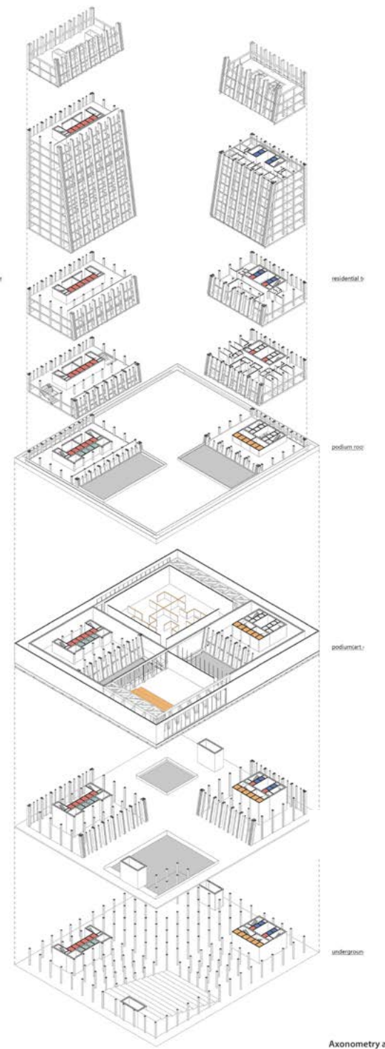
The Axonometric Drawing Public, apartment and office.
