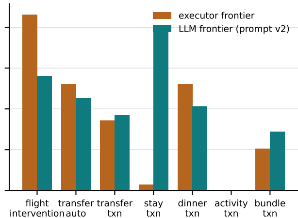
prompt v2: 73 episodes, k = 3 votes
