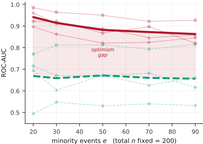
(a) Fix n , vary events r(\text{ceiling}, e) = -0.60
