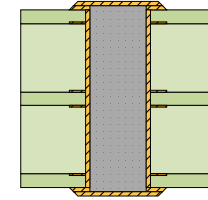
Via Type Type 7 (Scale 16:1)
