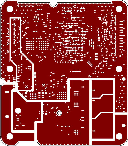
PWR4 (Scale 1:1)
