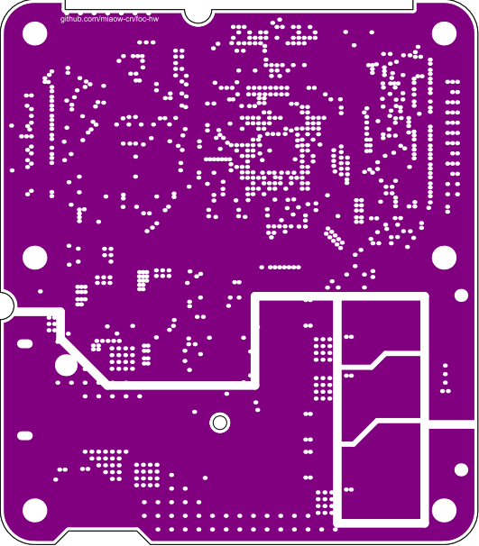
GND5 (Scale 1:1)
