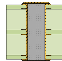
Via Type Type 7 (Scale 16:1)
