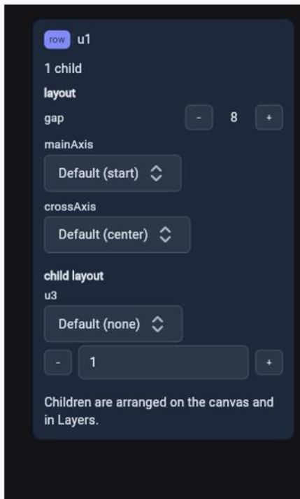
Row container: gap stepper, mainAxis, crossAxis, child expand + flex
