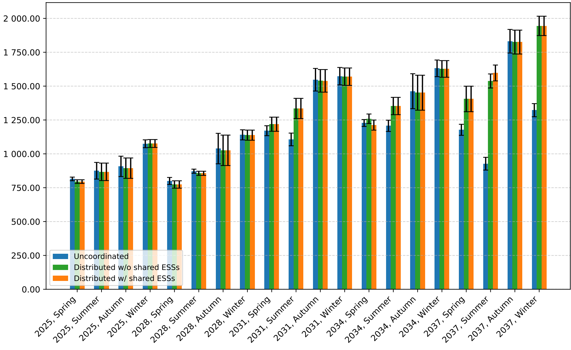
Renewable Generation, [MWh]
