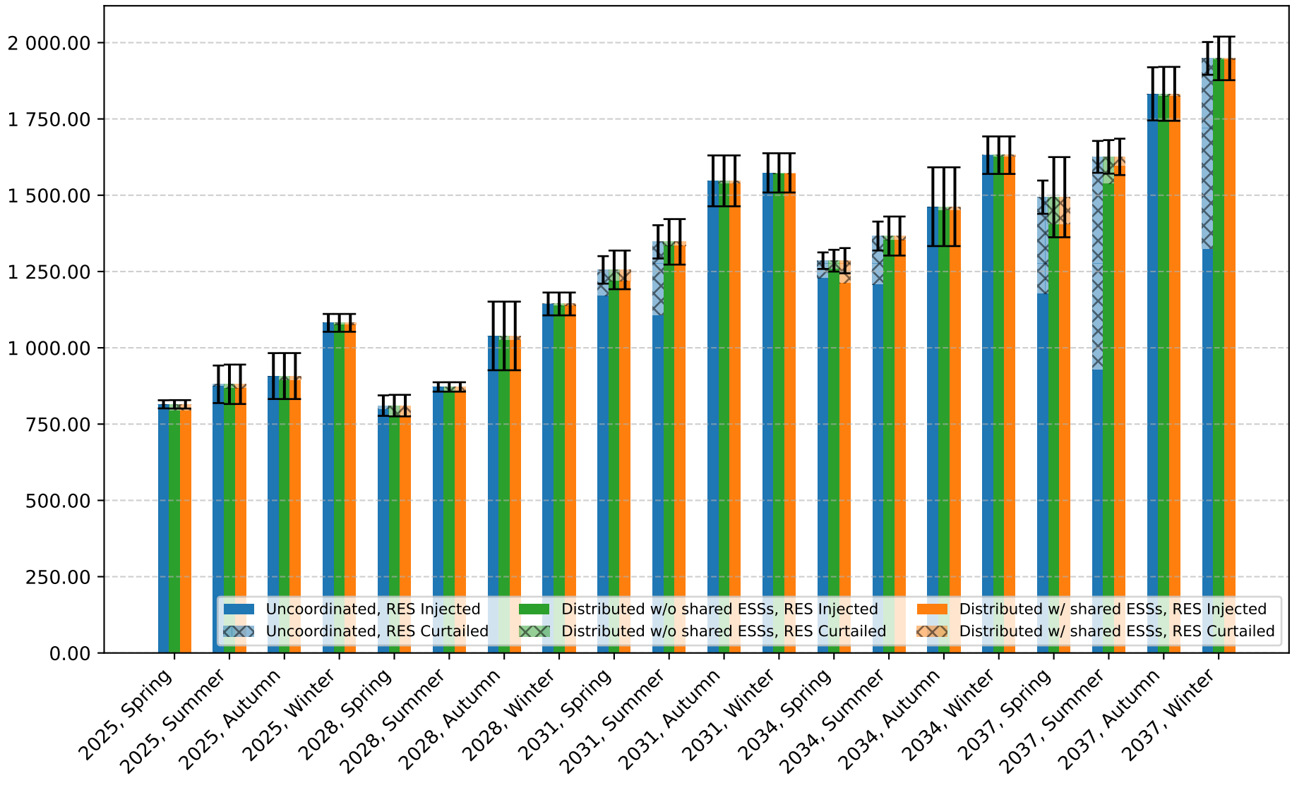
RES Generation, [MVAh]
