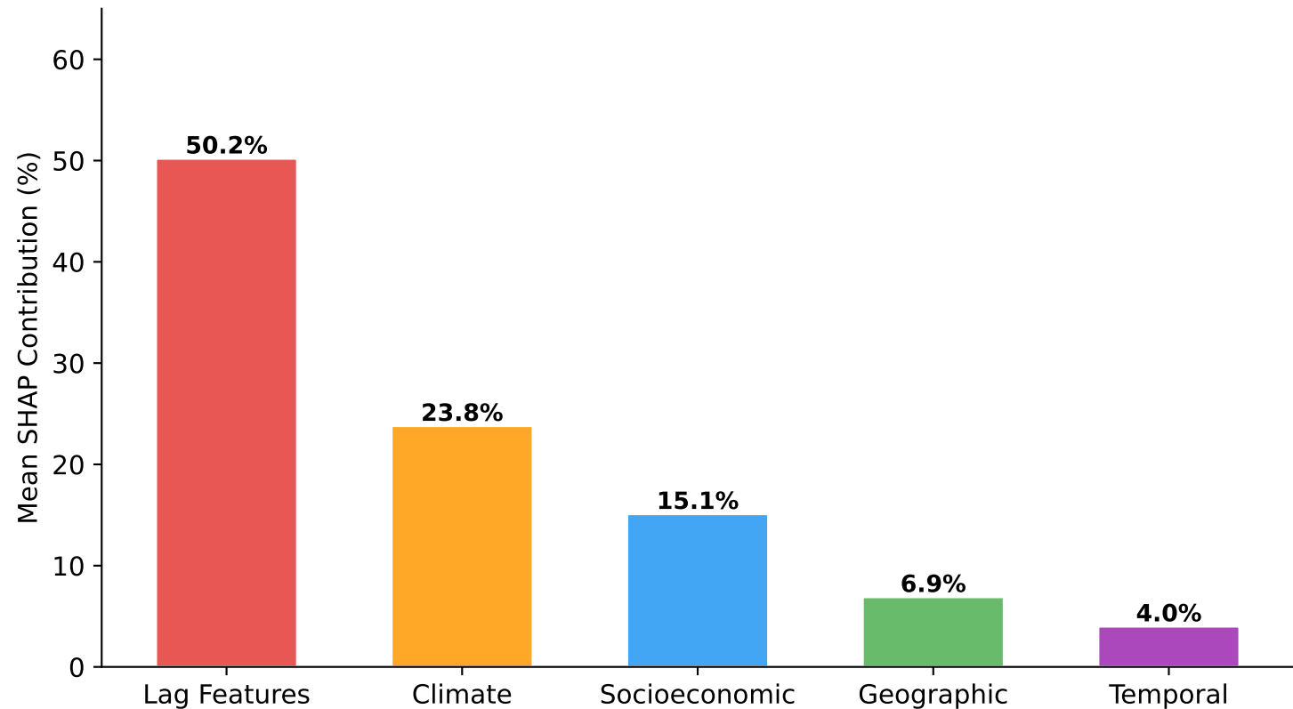
Figure 4.5: Feature Category Contributions (SHAP) Mean across all 8 diseases — RLRf model
