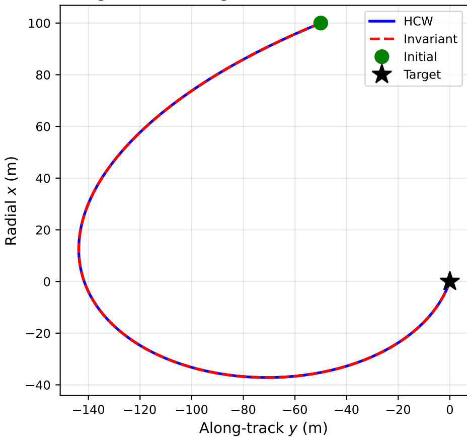
Figure 1: Coasting Circular-Orbit Rendezvous
