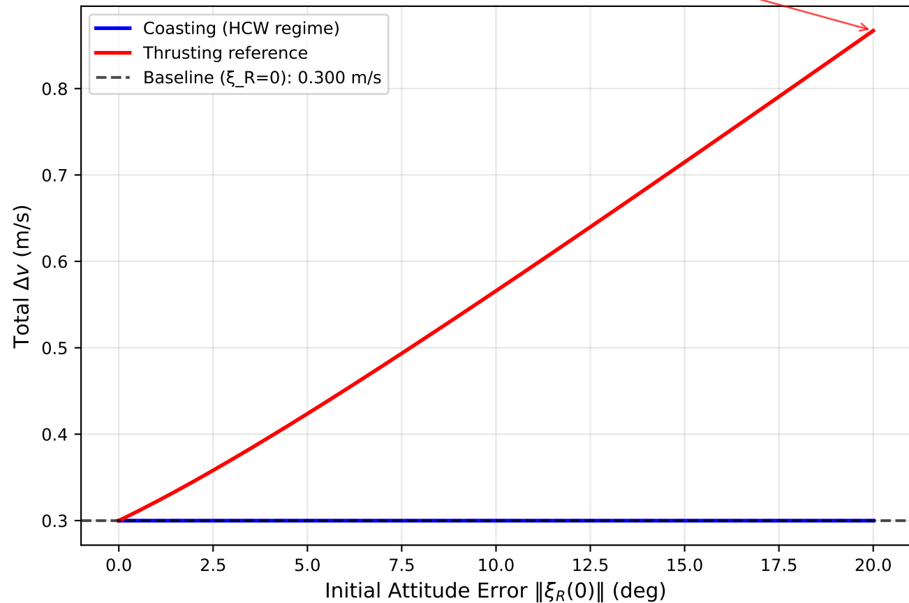
Figure 10: \Delta v Sensitivity to Attitude Error
