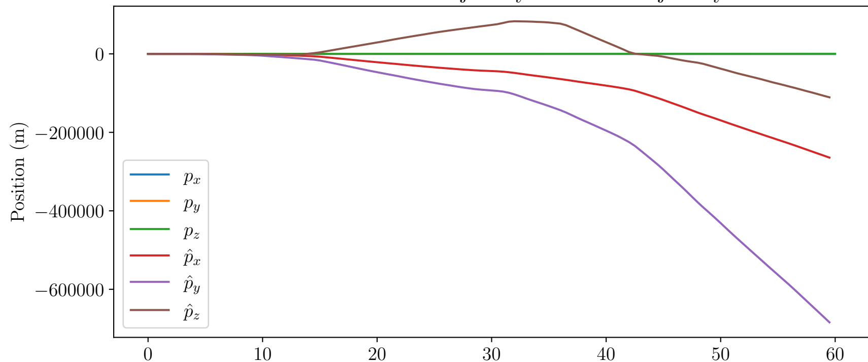
IEKF Estimated Trajectory vs. True Trajectory
