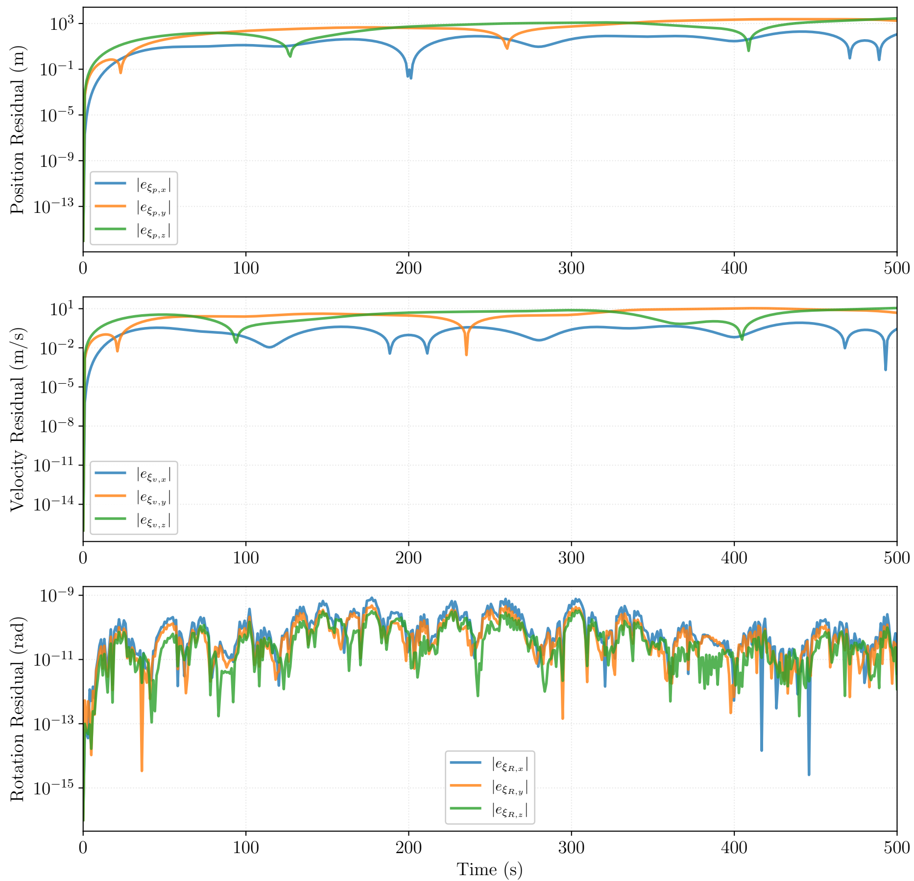
Residual e_\xi(t) = \xi_{nl}(t) - \xi(t) (Time-Varying Controls)
