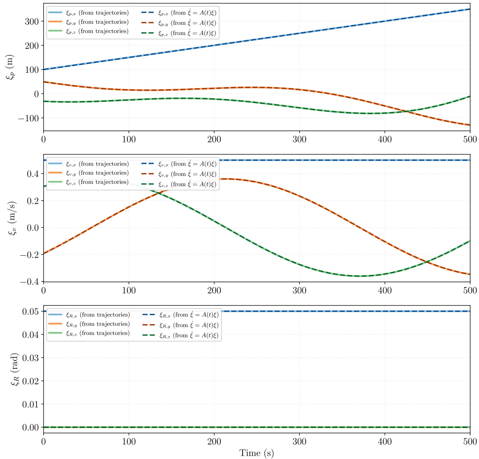
Exact Log-Linear Error Dynamics on SE_2(3)
