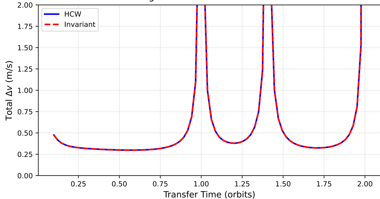
Figure 4: \Delta v vs Transfer Time
