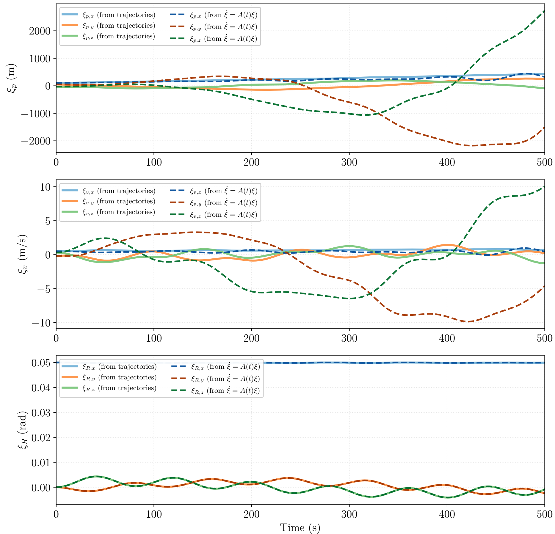
Exact Log-Linear Error Dynamics on SE_2(3) (Time-Varying Controls)
