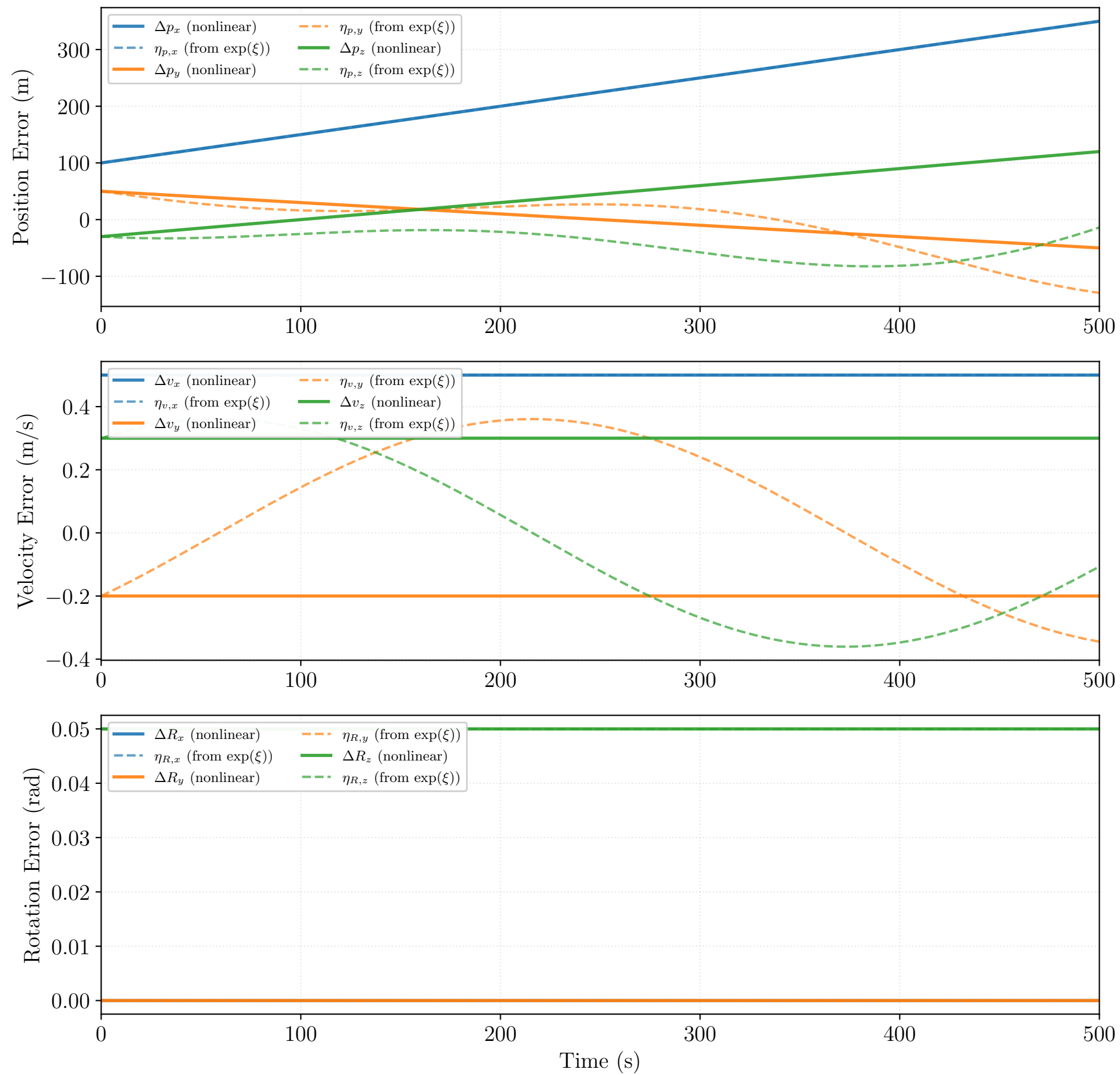
Euclidean Error vs. \eta = \exp(\xi) from Log-Linear Dynamics
