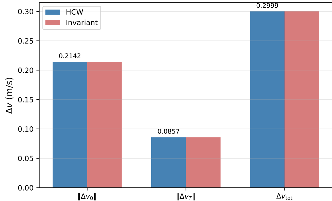
Figure 2: Two-Impulse \Delta v Comparison
