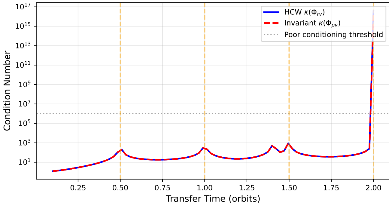
Figure 5: Conditioning of Boundary-Value Solve
