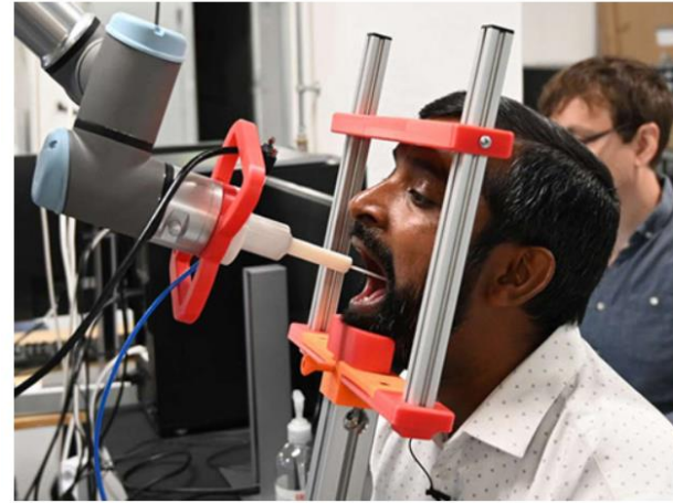
Coron-19 Test Robot@SDU(Uni. of Southern Denmark)
