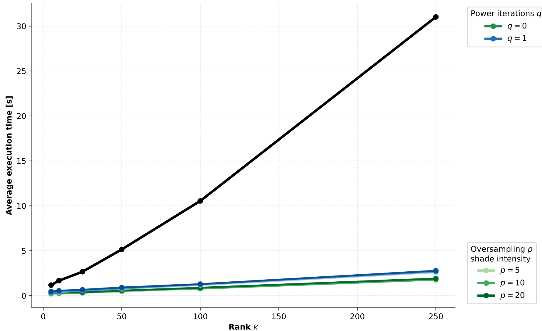
Image compression: average rSVD execution time
