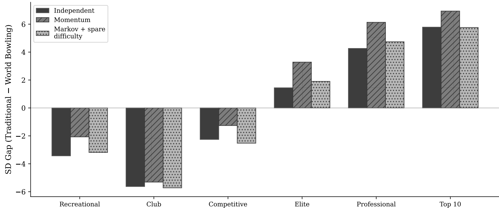
Traditional Scoring Advantage: Three Simulation Models
