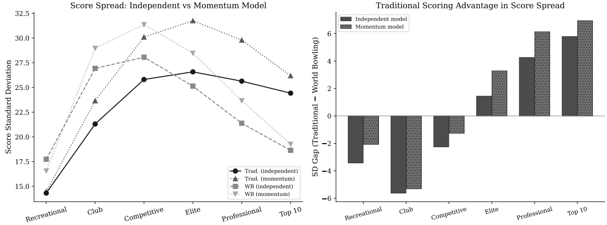
Figure 11: Left: score standard deviation under independent and momentum models. Right: the SD gap between systems widens under momentum at elite tiers.
