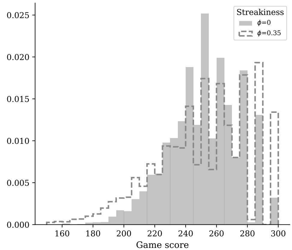
World Bowling ( d = -0.02 )
