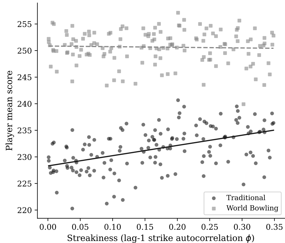
Same marginal skill, different streakiness (Trad. r = +0.49 , WB r = -0.04 )
