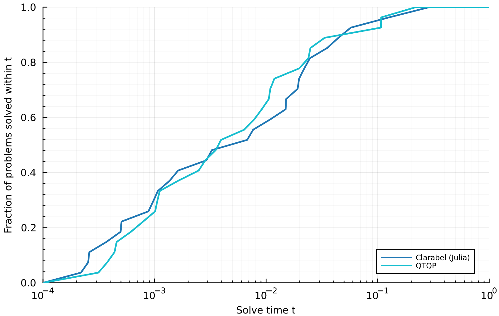
Solution time profile
