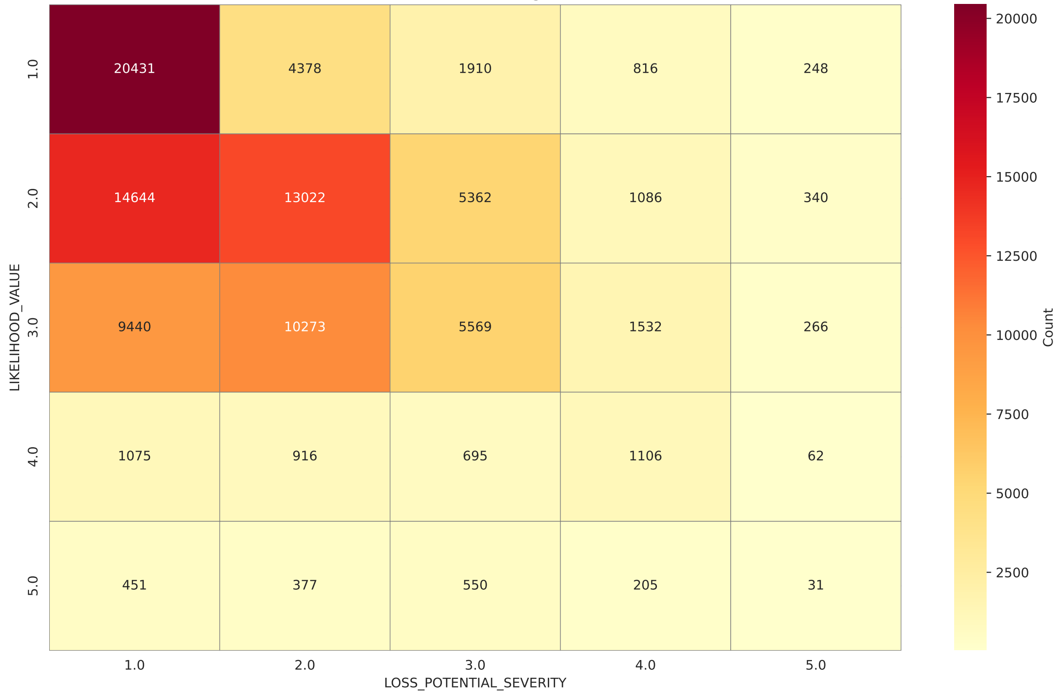
Severity vs Likelihood Heatmap (Valid: 94,785, Missing: 3,771)
