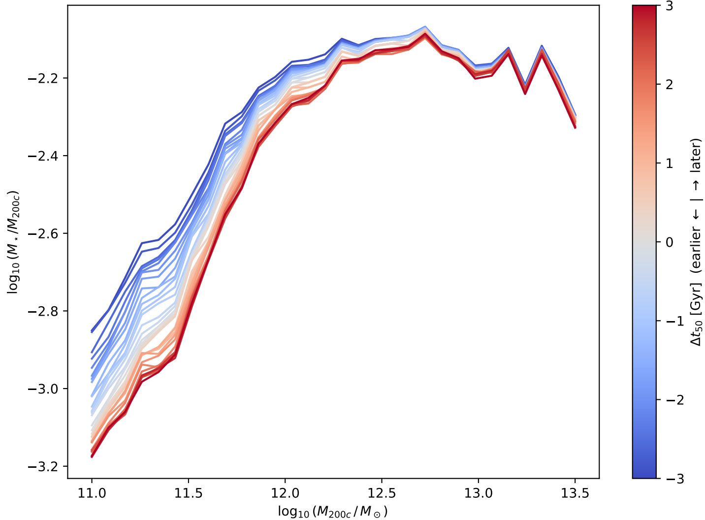
Emulated SHMR vs shift in t_{50}
