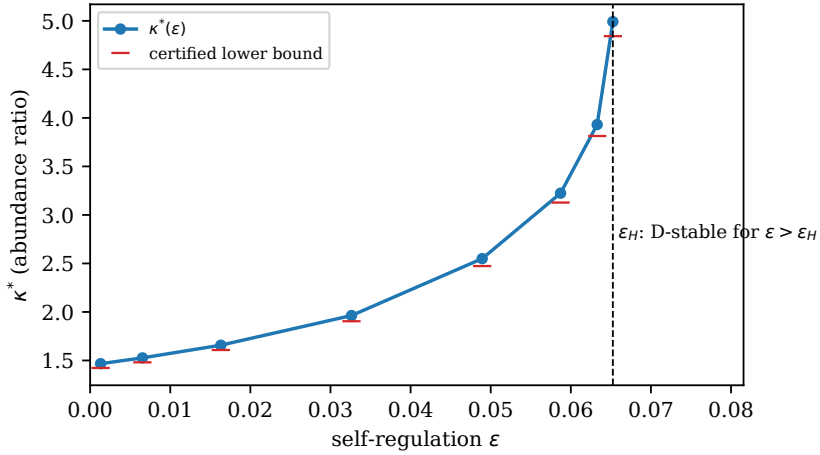
Figure 2: Section 7.1: \kappa^*(\varepsilon) on (0, \varepsilon_H] with the certified lower bounds. D-stability holds exactly for \varepsilon > \varepsilon_H ; stability at equal abundances holds on the whole interval shown.
