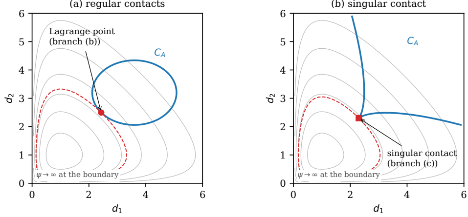
Figure 1: Schematic of the coverage argument, drawn in two dimensions (the contact set itself has dimension n-2 ). Grey: level sets of \psi(d) = \sum_i (d_i - \log d_i) , which blow up at the boundary of the orthant. Blue: contacts. The minimizer of \psi over the contacts is either a regular point where a level set touches C_A (a solution of (b), panel (a)) or a singular point of C_A (a solution of (c), panel (b)).
