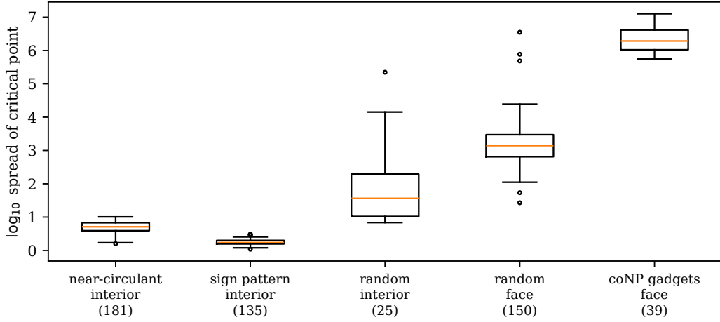
Figure 3: Certified boundary atlas: spread of the \psi -minimal critical point at the unstable endpoint of a certified bracket (an upper bound for \kappa^* ), by matrix class and birth type, for the 530 of the 538 brackets of Section 8 whose critical point was recorded; counts in parentheses. The classes are defined in Section 8.
