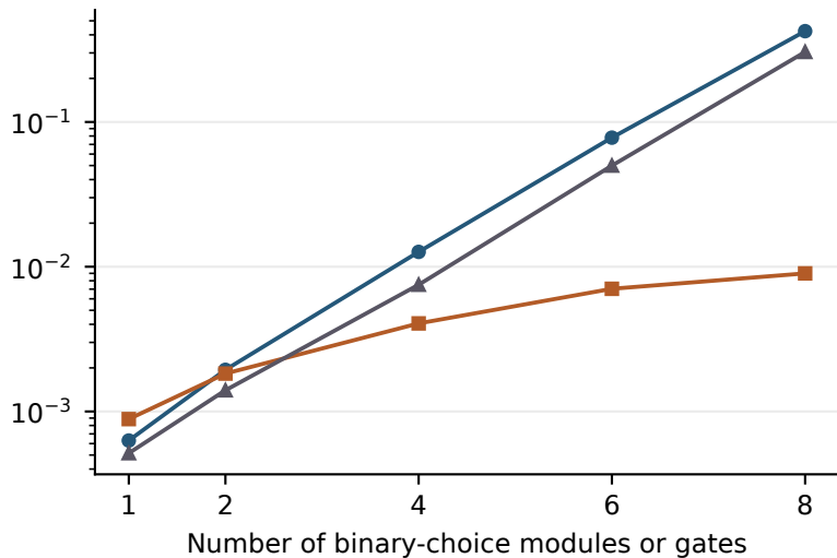
Construction time (s)
