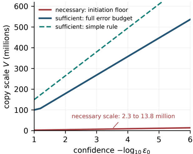
(b) copy scale versus target failure \epsilon_0
