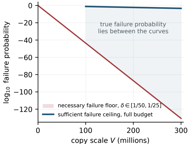
(a) H = 100 windows, bounds versus V
