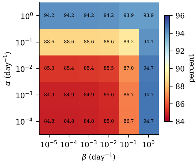
independent-founder limit 2\Phi(z_{.975}\sqrt{v_Z/v_N}) - 1
