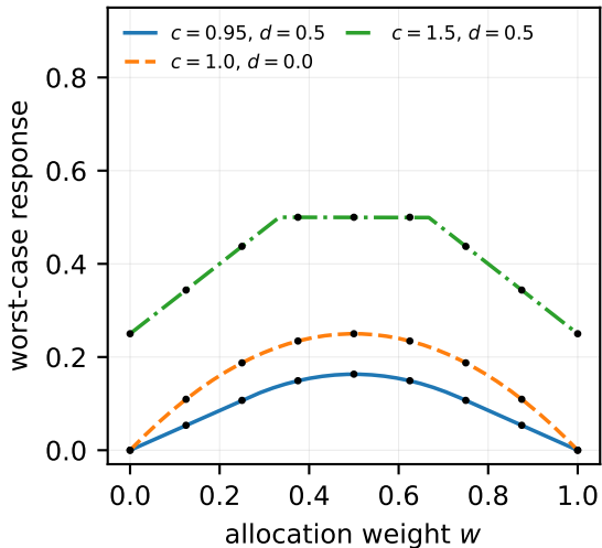
A. exact profile (dots: brute force)
