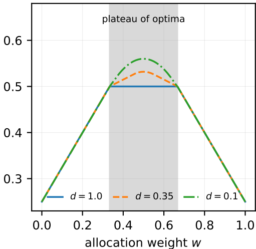
B. non-binding budget flattens the optimum ( c = 1.5 )
