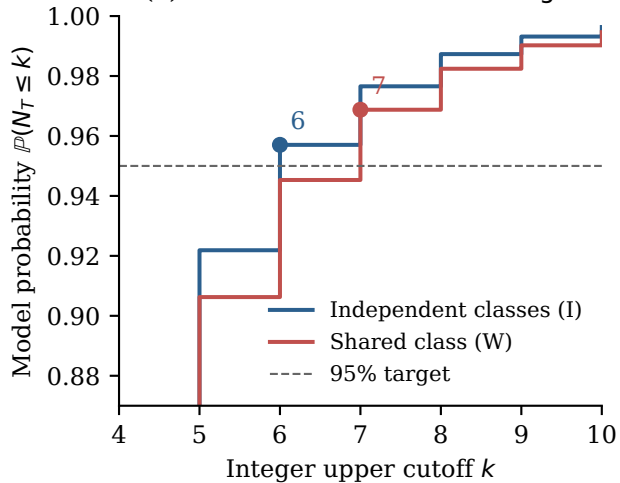
(a) Two-founder CDFs at T = \log 2
