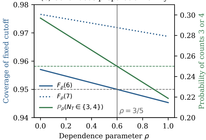
(b) Continuous preparation family
