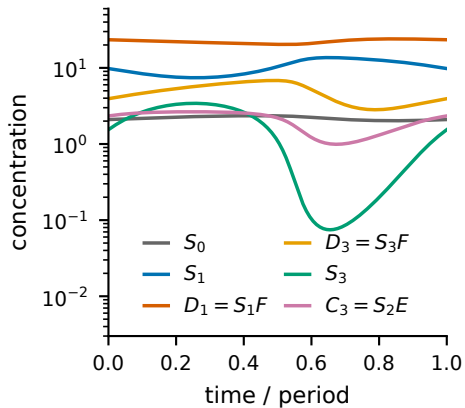
(b) one period, r = 1
