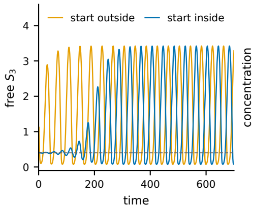
(a) convergence to the cycle, r = 1
