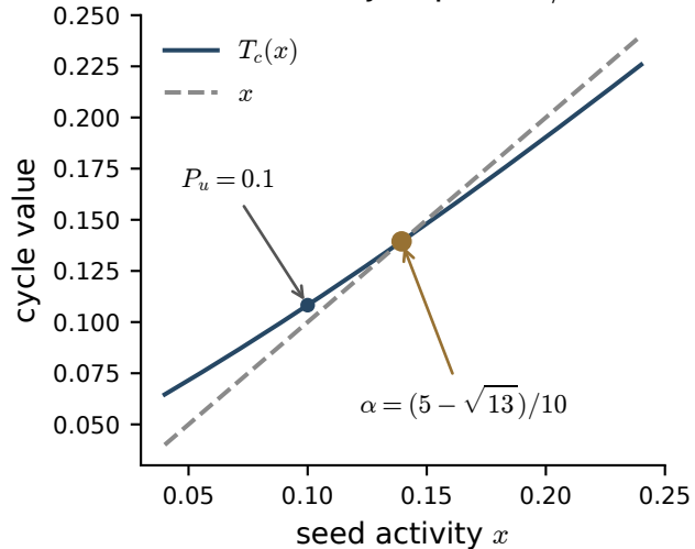
(a) forced jump, t = 1/100
