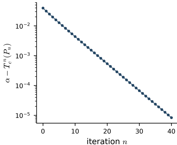
(b) plain iteration never lands
