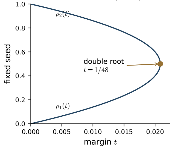
(c) branches of x(1 - x) = 12t
