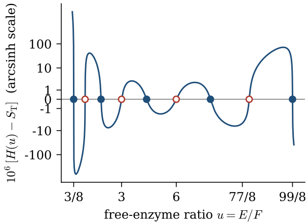
(b) n = 5, r = 13 : nine steady states
