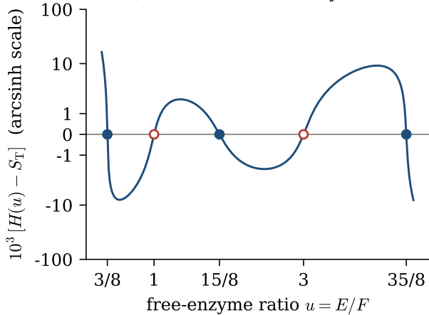
(a) n = 3, r = 5 : five steady states
