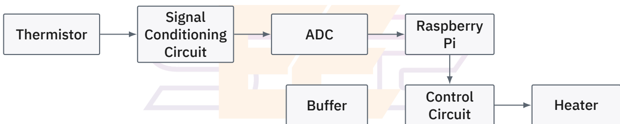
Figure 8.1: Block diagram of the temperature control system.
