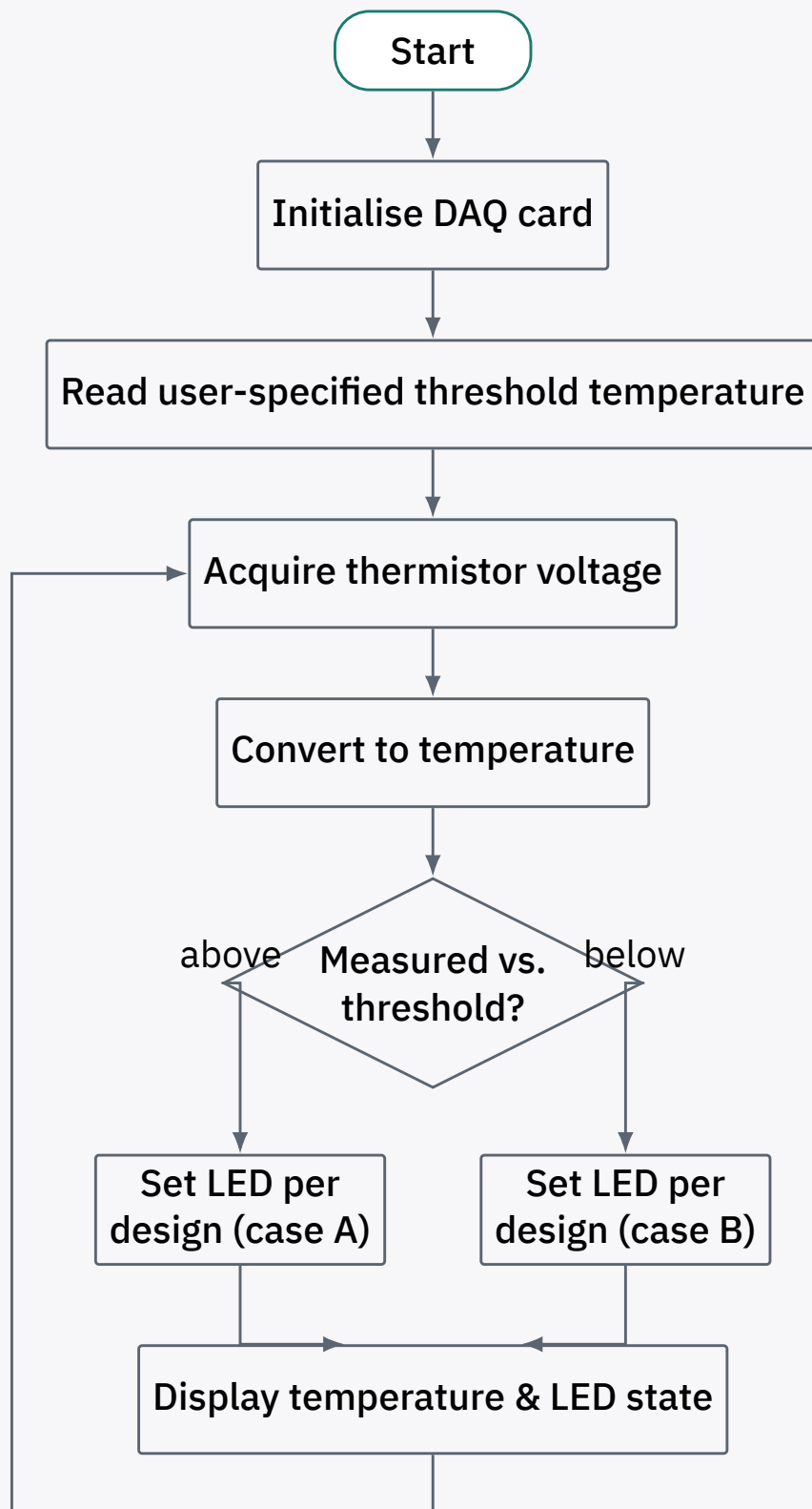
Figure 16: Temperature monitoring and LED control loop (ON/OFF direction per student design).
