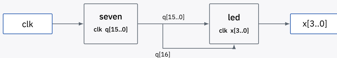
Figure 8: Schematic diagram for the 16-bit binary counter with frequency divider.
