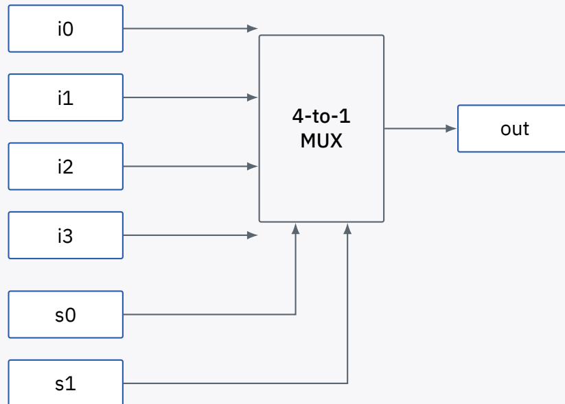
Figure 4: Schematic-entry 4-to-1 multiplexer (mux_sch).
