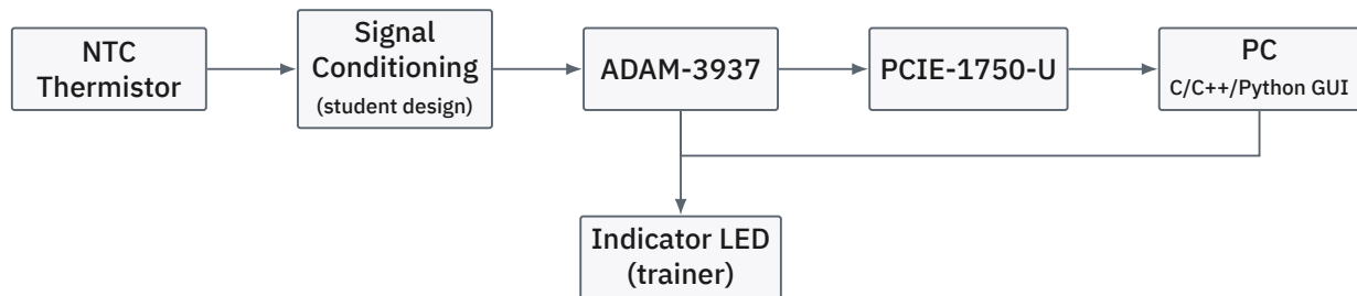
Figure 15: Block diagram of the temperature measurement and control system.
