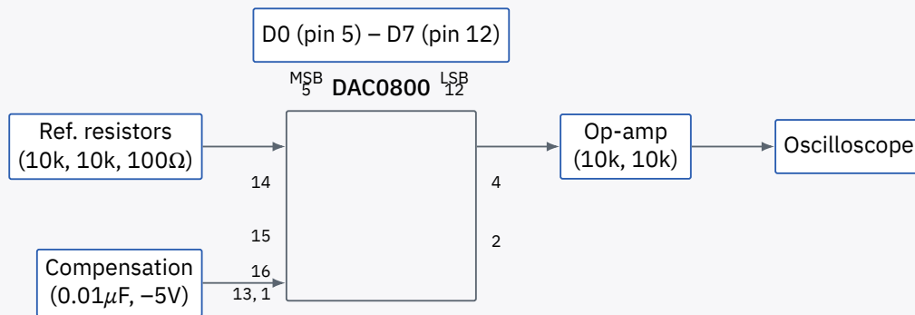
Figure 19: DAC0800 test circuit with op-amp output stage.
