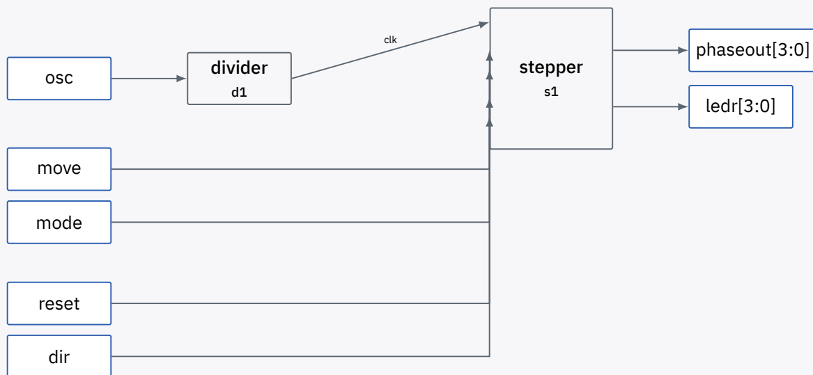
Figure 11: RTL Viewer overview of the step top-level module.
