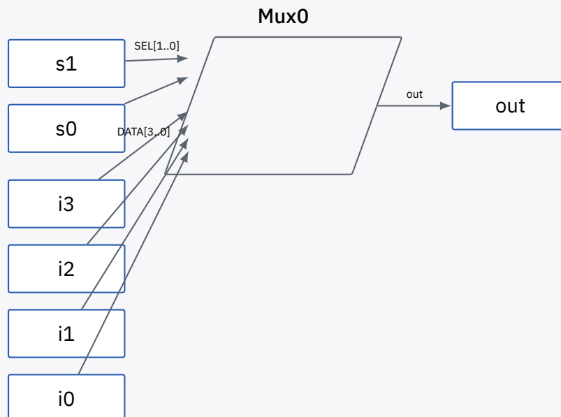
Figure 5: RTL Viewer output for mux_ver (Mux0).
