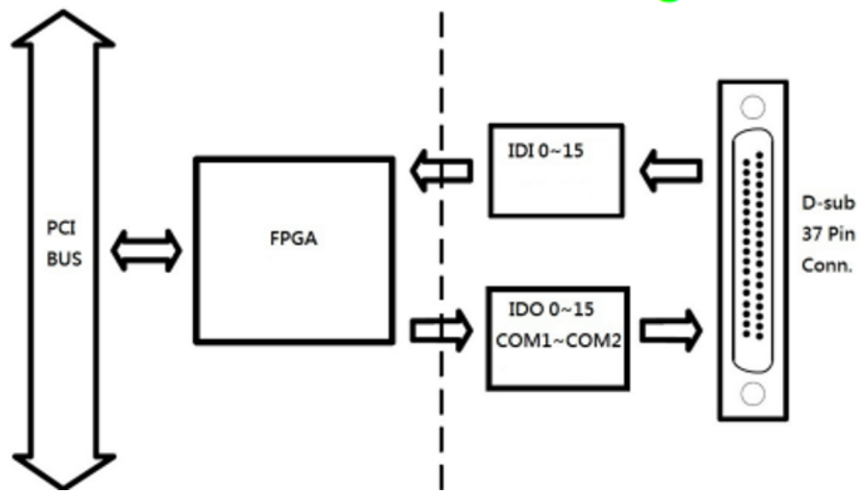
Figure 7.4: PCI-1750/PCI-1750SO block diagram (PCI-1750 user manual, p. 9).
