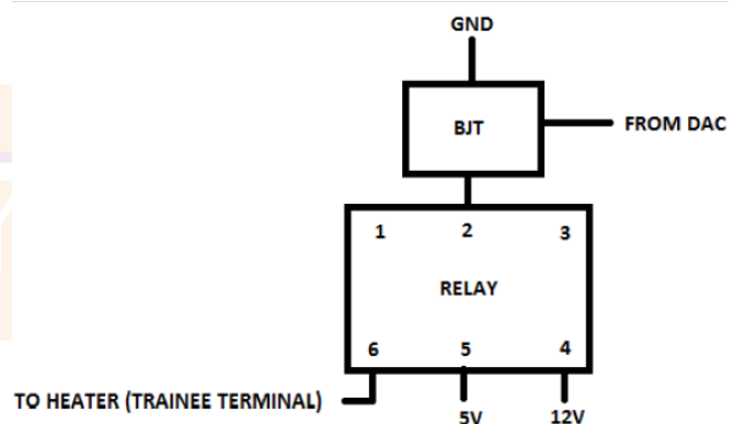
(b) connection diagram
