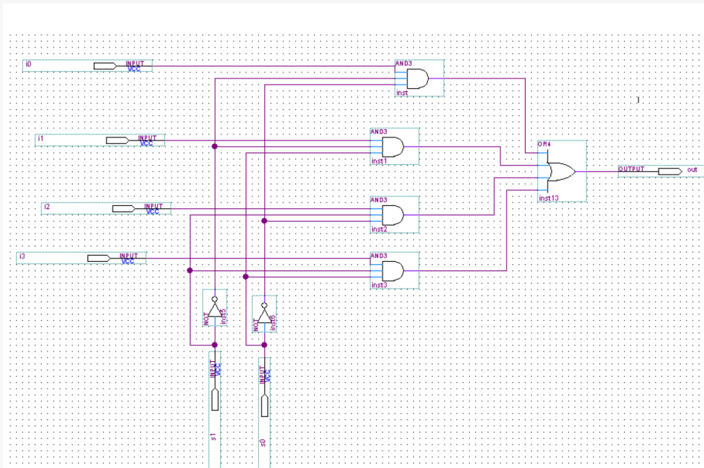
Figure 5: Mux Schematic.
