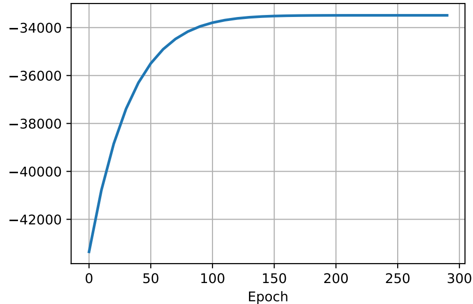
BTL Likelihood
