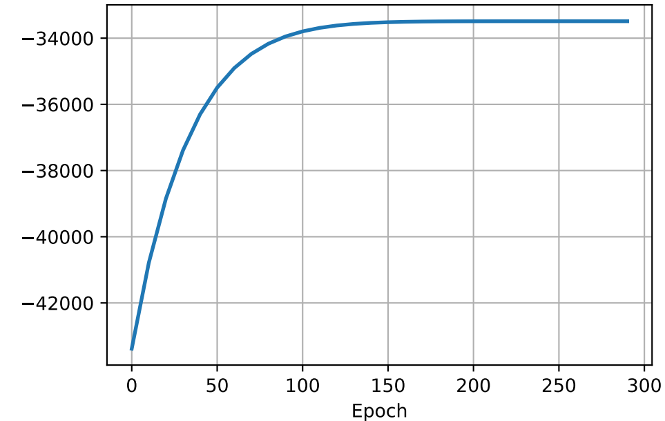
Total Likelihood
