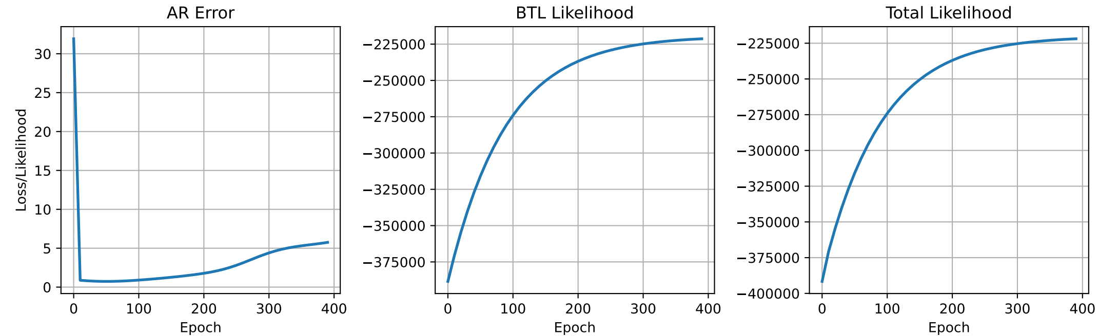
AR Error, BTL Likelihood, and Total Likelihood (std=0)
