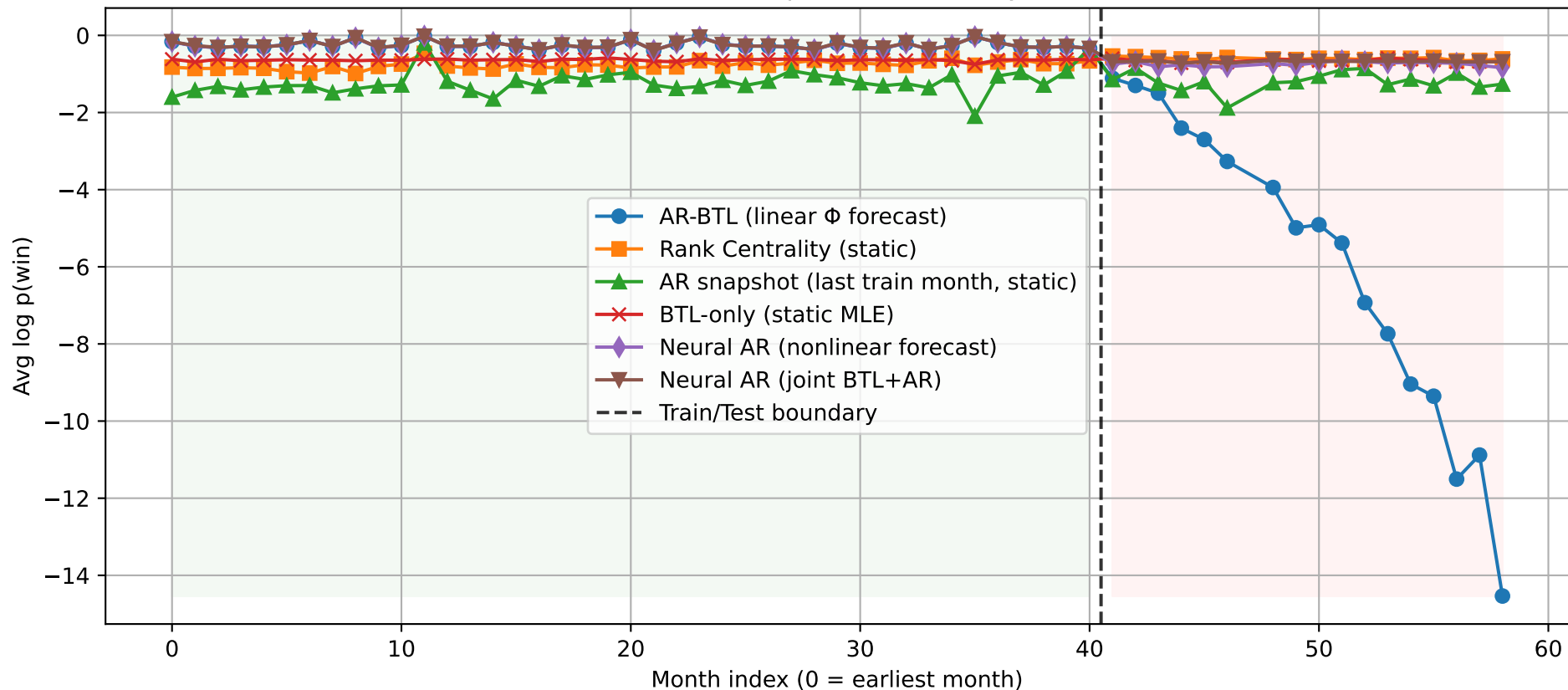
Per-month predictive log-likelihood: AR-BTL vs RC vs AR-snapshot vs BTL-only vs Neural-AR
