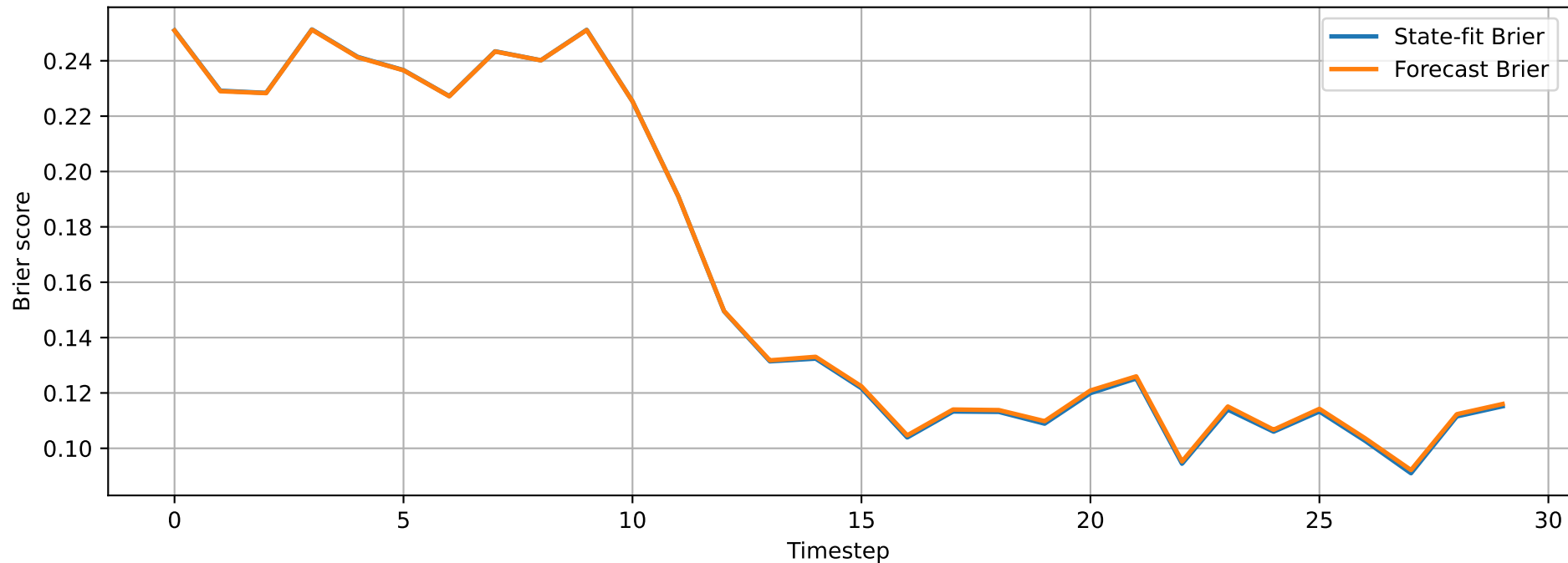
BTL Probability Error: Weighted Brier (lower = better)
